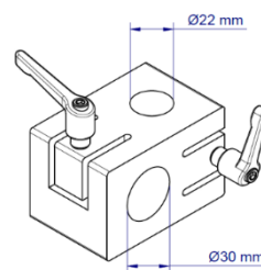
TBMA8-PAT, shaft to shaft
