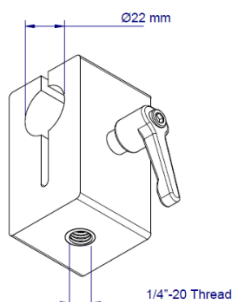
TBMA4-PAI, thread to shaft
