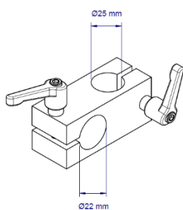
TBMA4-PAT, shaft to shaft
