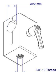
TBMA4-PAI-3-8, thread to shaft
