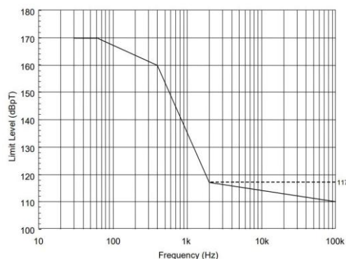
RS101 limits for all Navy & Army applications
