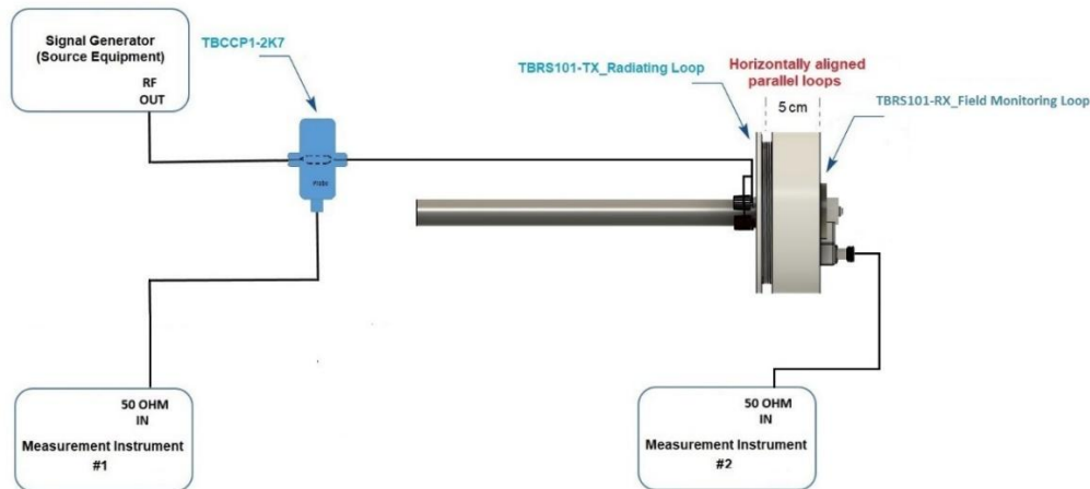
TBRS101 Typical Calibration Setup (RF Current Probe Method)
