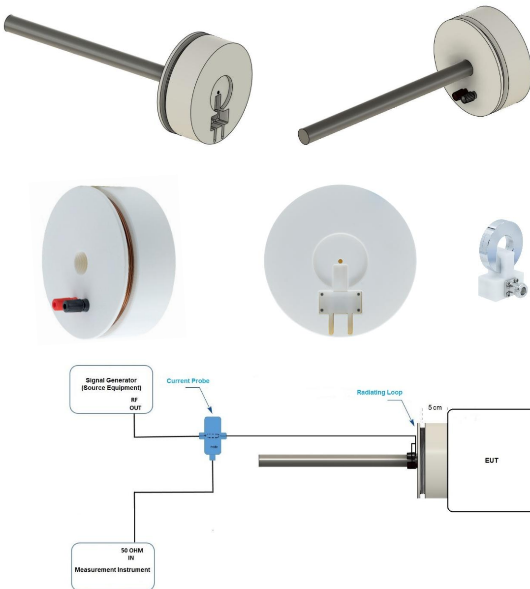
TBRs101 Typical Test Setup
