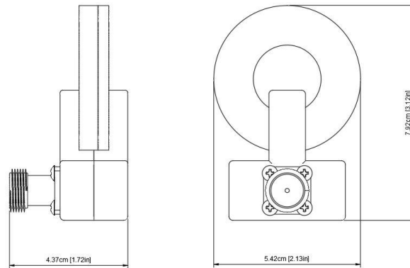
Dimensions of TBRs101-RX field monitoring loop
