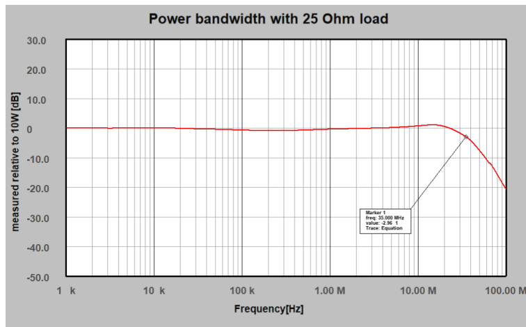
Figure 3 - Example: 3 dB Power bandwidth with 25 Ohm load: 35 MHz
