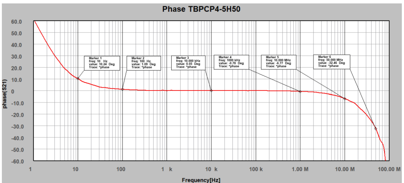
Figure2: S21, phase, 1 Hz – 100 MHz
