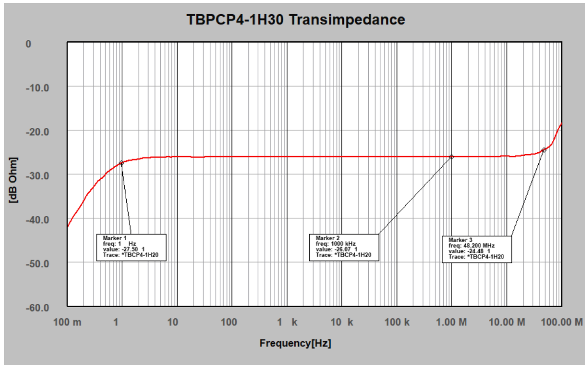
Figure1: typical transfer impedance, 1 Hz – 100 MHz
