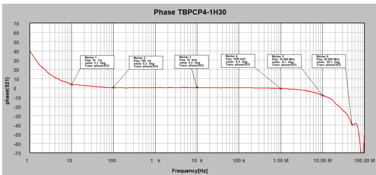
Figure2: S21, phase, 1 Hz – 100 MHz
