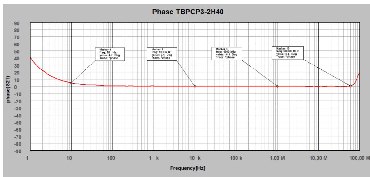
Figure2: S21, phase, 1 Hz – 100 MHz
