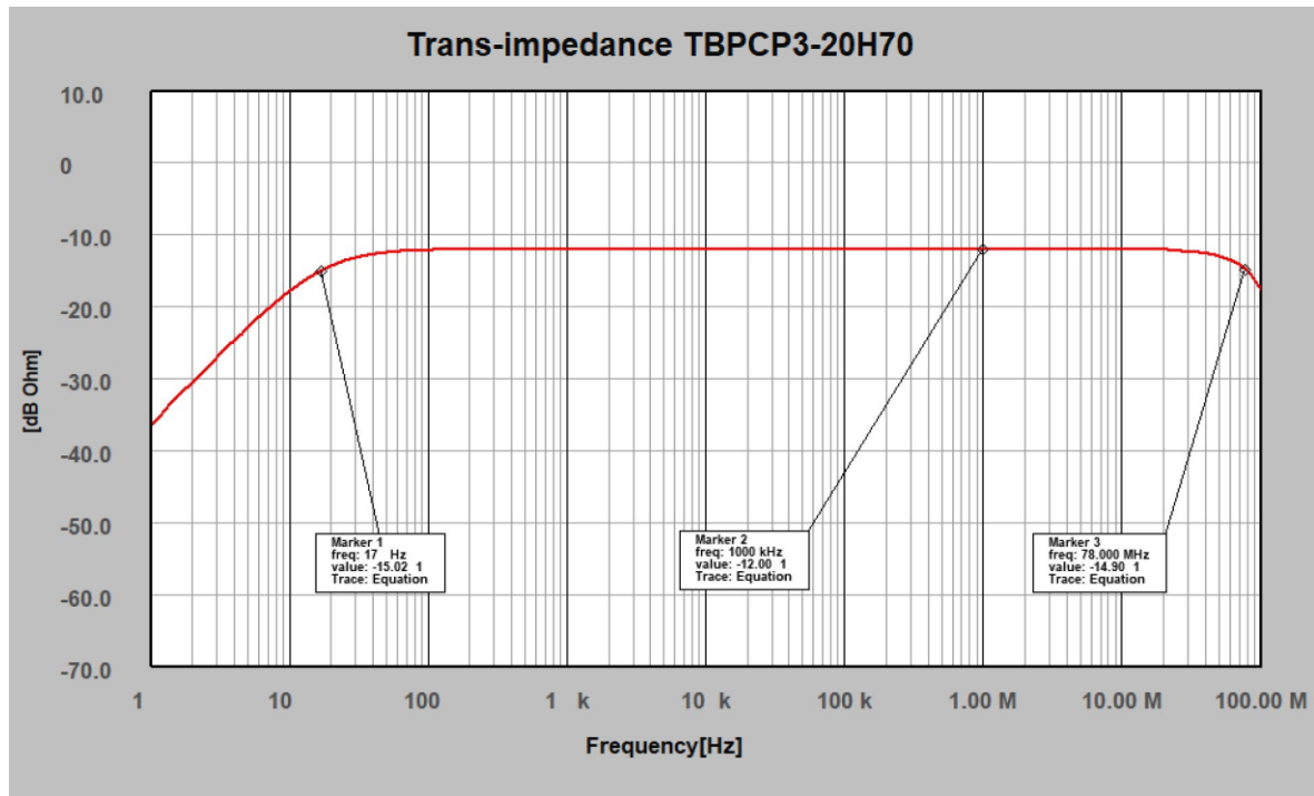
Figure1: typical transfer impedance, 1 Hz – 100 MHz
