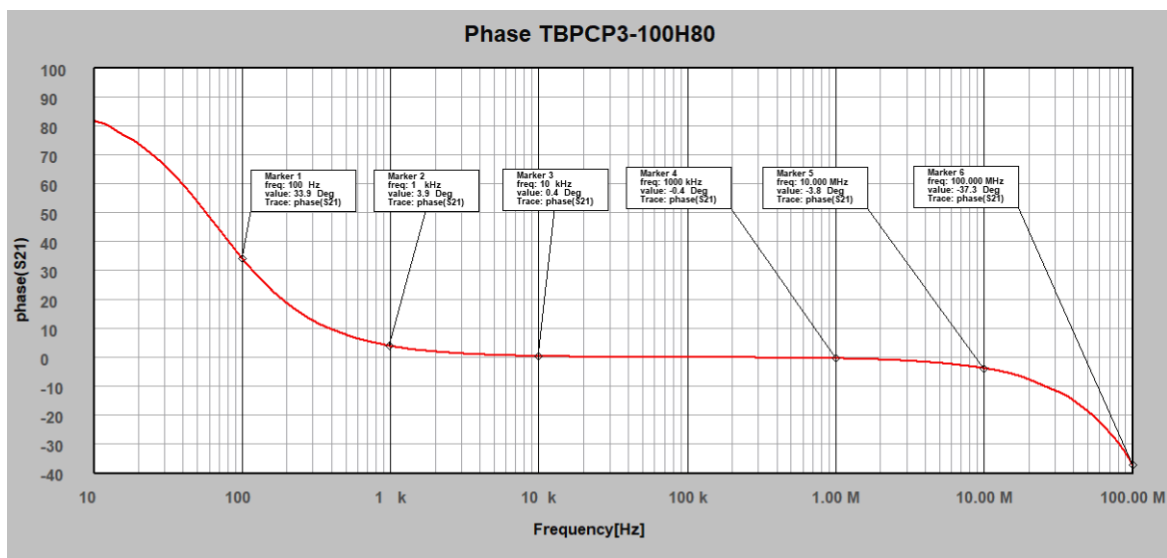
Figure 2: S21, phase, 10 Hz – 100 MHz
