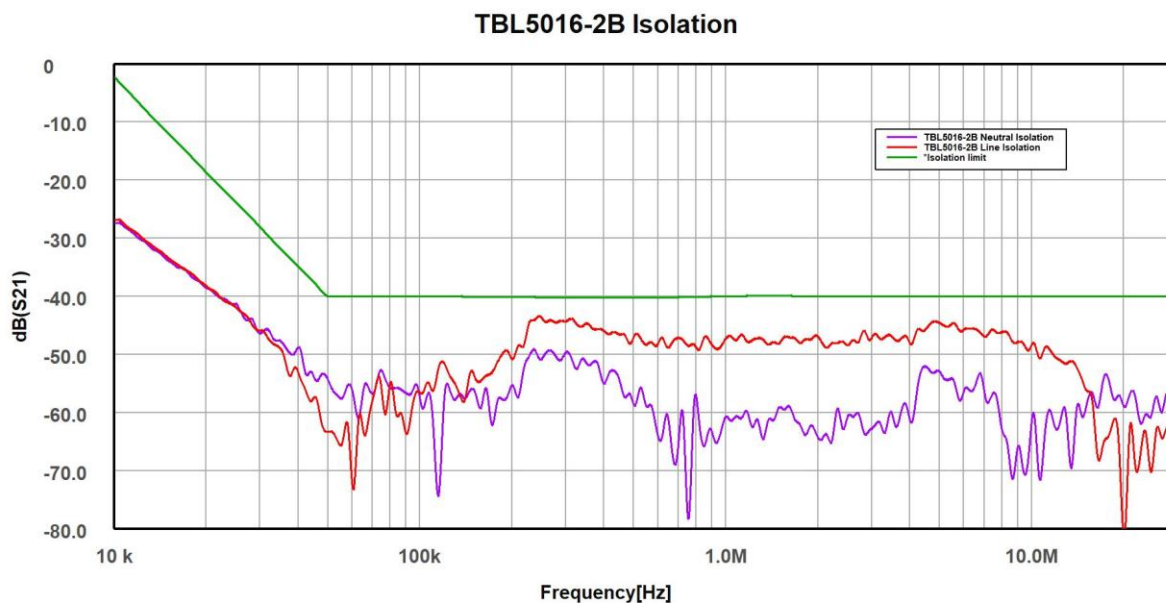
LISN Isolation, Source to RF out, typ.
