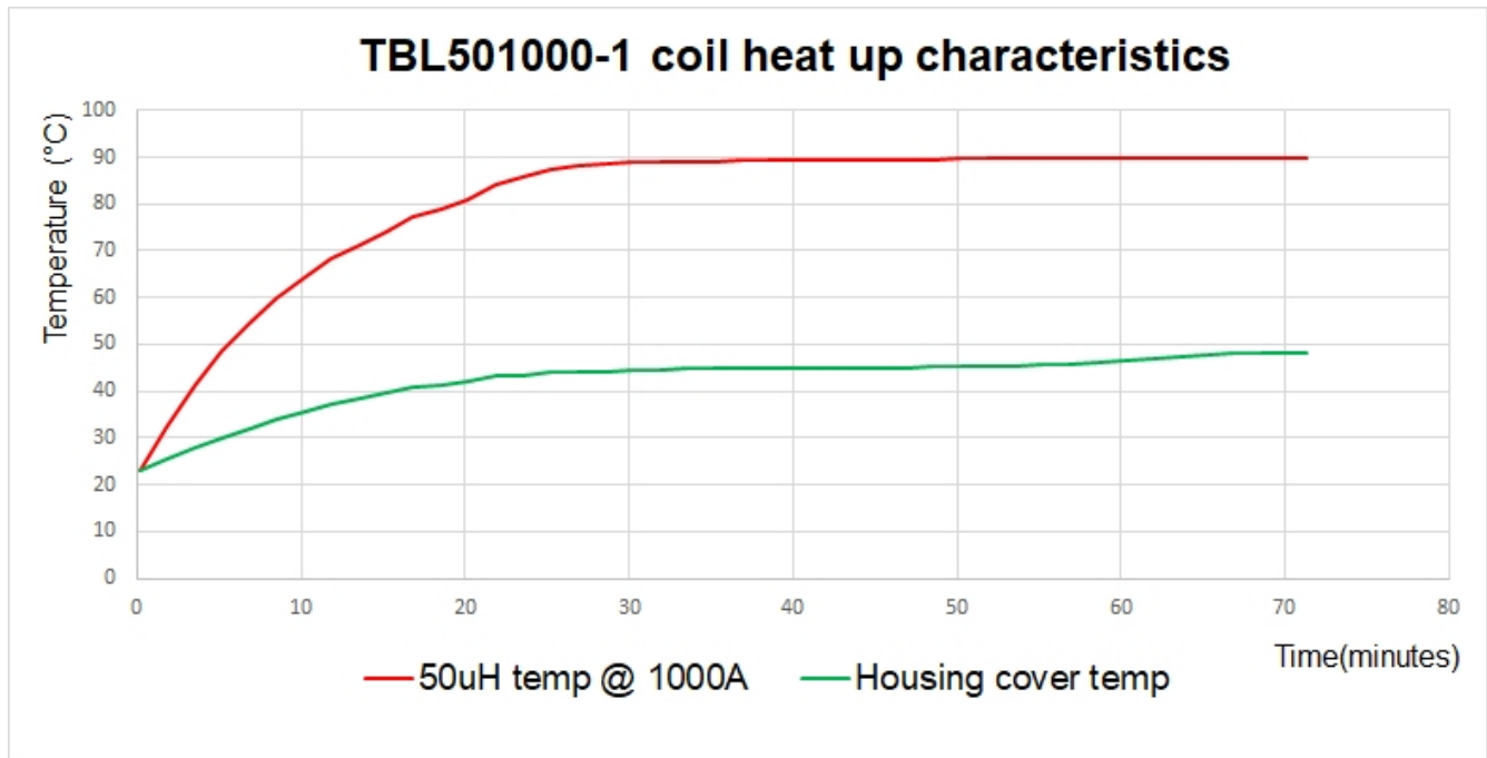
Picture 6: Coil and housing temperature at 1000 A AC current, 50 Hz, fan ON
