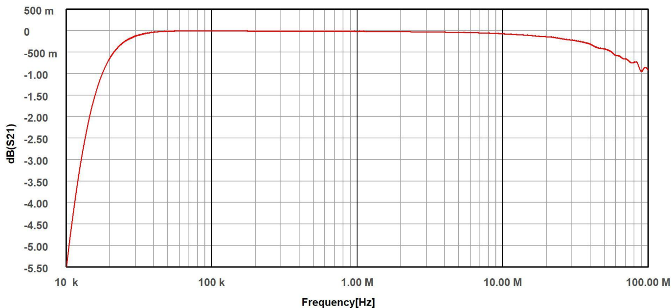
TBL50100-1B Voltage Division Factor (50uH + 5 Ohm) // 50 Ohm
