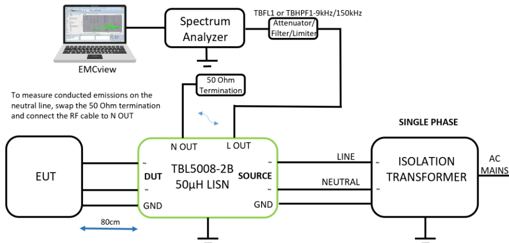
Basic wiring diagram for conducted emission measurements
