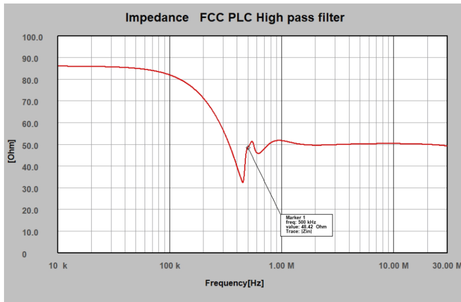
TBHPF1-500kHz: Impedance, 10 kHz to 30 MHz, typical data
