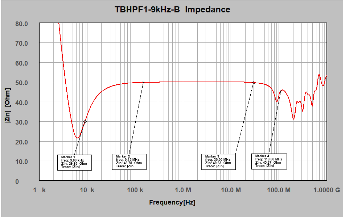
TBHPF1-9kHz-B: Impedance, 1 kHz to 1 GHz, typical data
