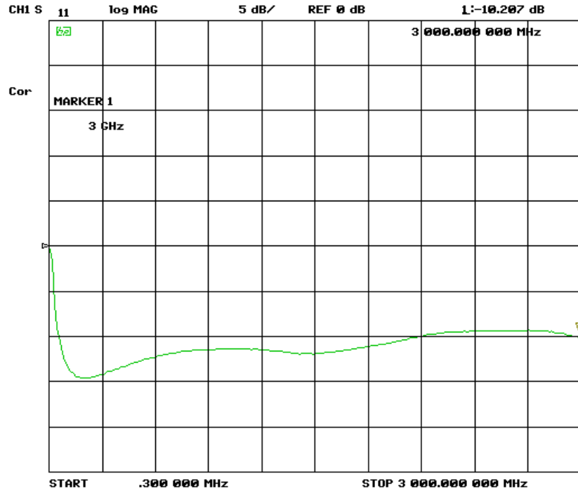
Picture 11 – TBDA1/28dB, input return loss, S_{11} , 300 kHz – 3 GHz, lin.
