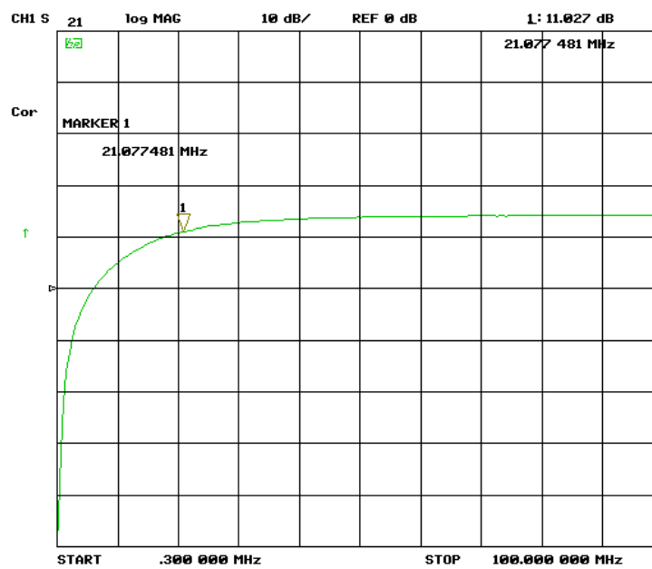
Picture 3 – TBDA1/14dB, gain, 300 kHz – 100 MHz, lin.
