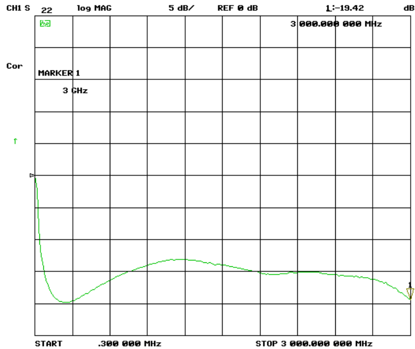
Picture 12 – TBDA1/28dB, output return loss, S_{22} , 300 kHz – 3 GHz, lin.
