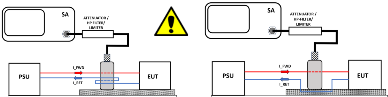
Figure 4: setups resulting in bias currents
