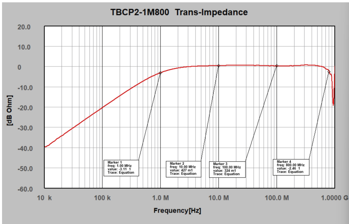
Figure1: typical transfer impedance: 10 kHz to 1 GHz
