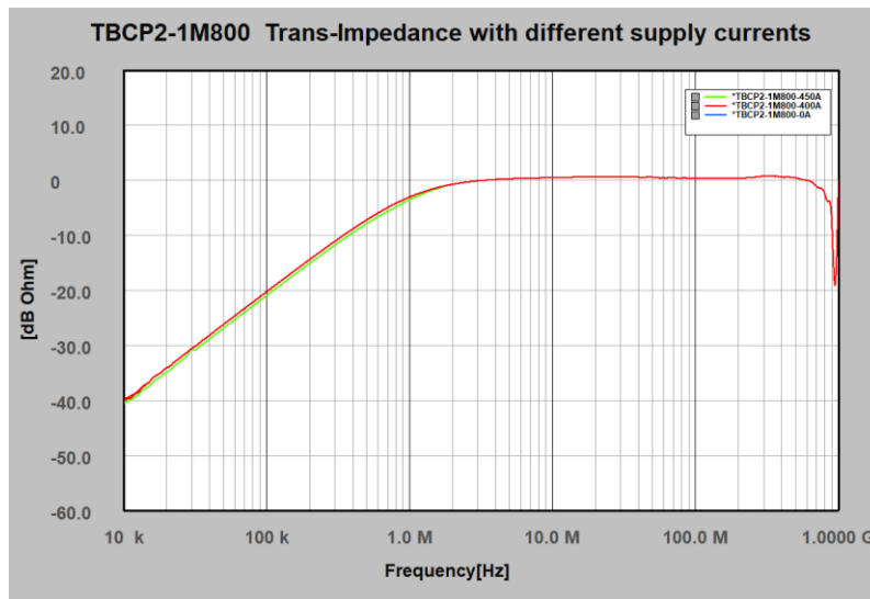
Figure2: transfer impedance versus supply current
