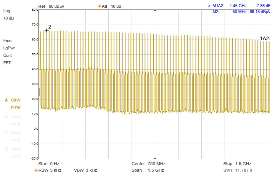
Figure 1 - f_{comb} : 10 MHz; 66 dBμV @ 50 MHz; spectrum flatness up to 1.5 GHz: -8dB
