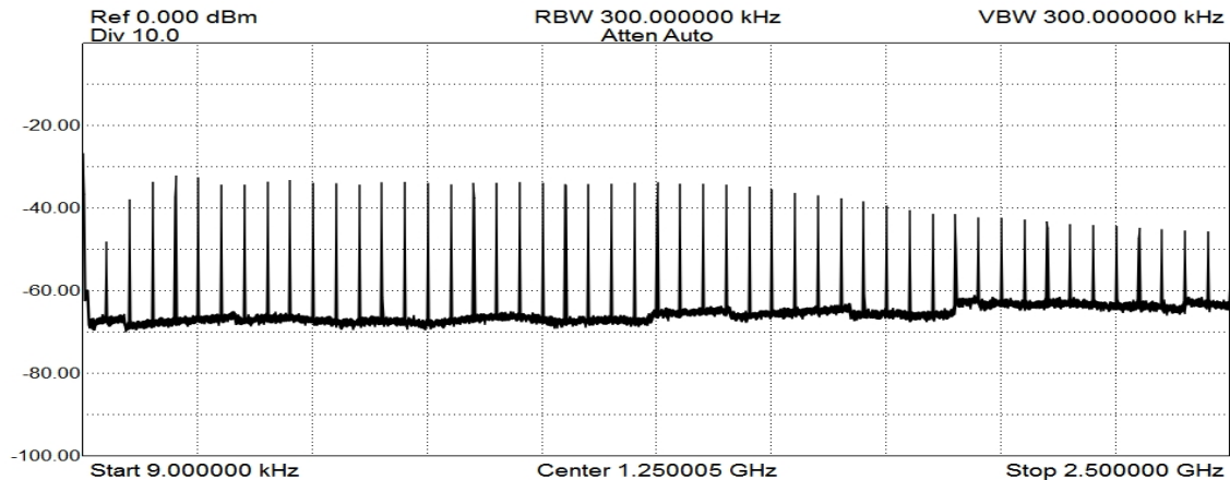
Output spectrum: input signal 50 MHz / +8dBm
