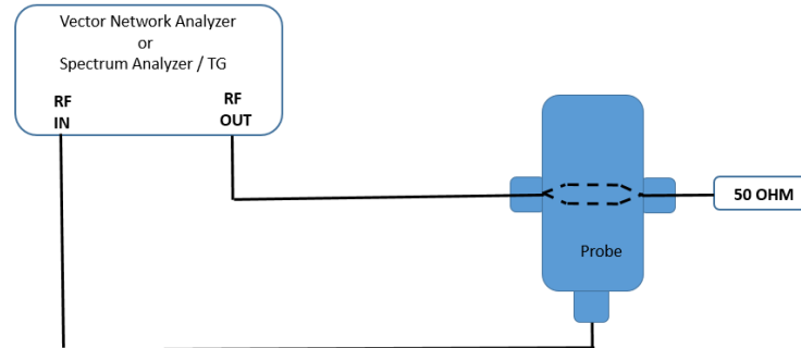
Figure 4: S 21 , transimpedance measurement set up
