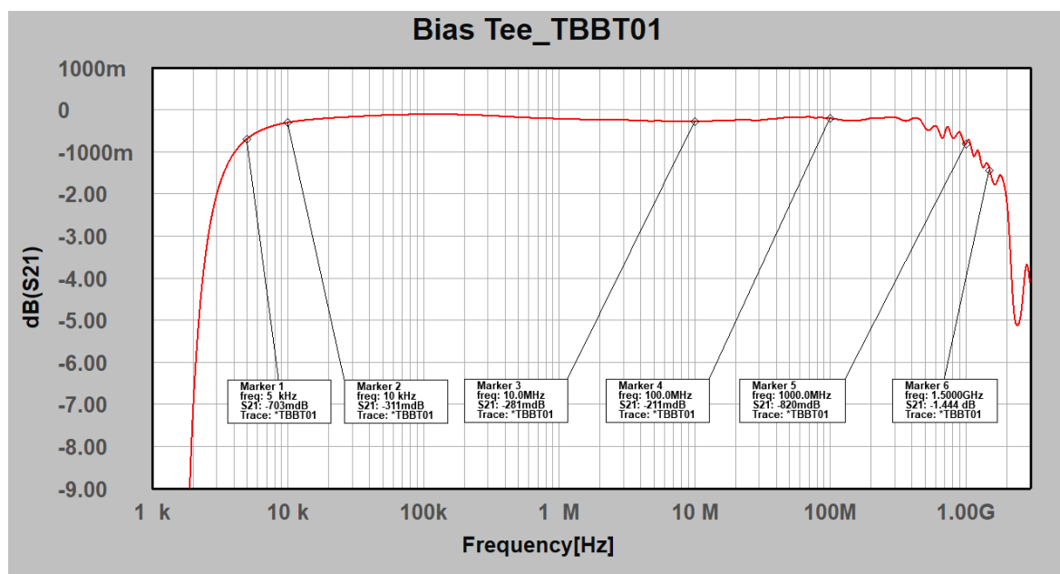
TBBT01, Insertion Loss, 1 kHz – 3 GHz
