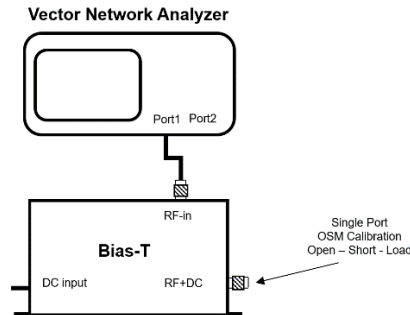
Calibration setup
