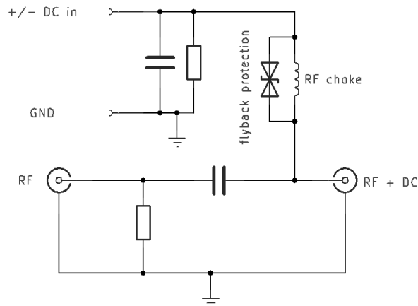
Simplified schematic of the TBBT01
