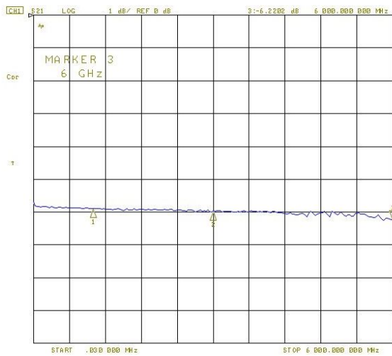
6dB Attenuator, S21 / VSWR
