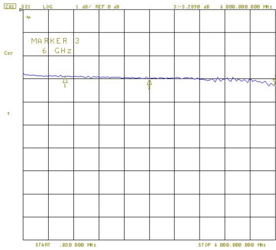
3dB Attenuator, S21 / VSWR
