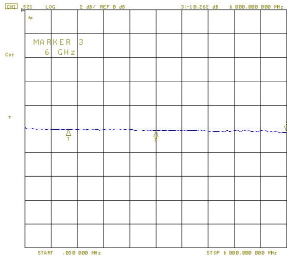
10dB Attenuator, S21 / VSWR
