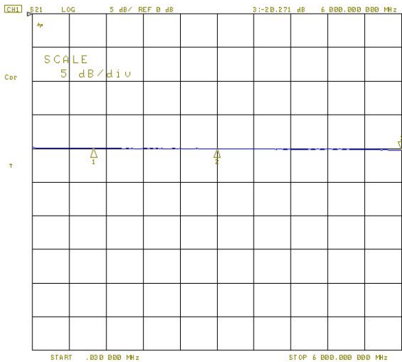
20dB Attenuator, S21 / VSWR
