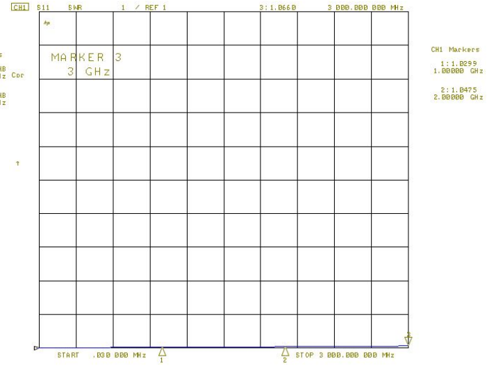
20dB Attenuator, S21 / VSWR
