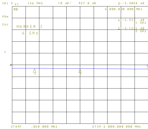
3dB Attenuator, S21
