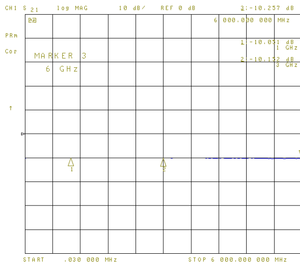
10dB Attenuator, S21
