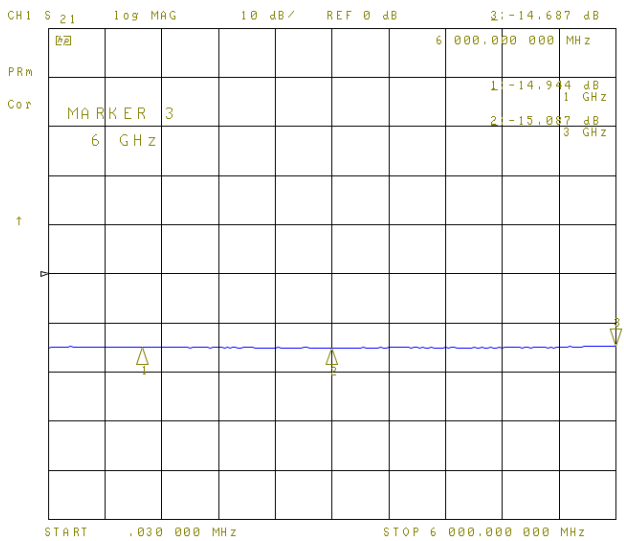
15dB Attenuator, S21
