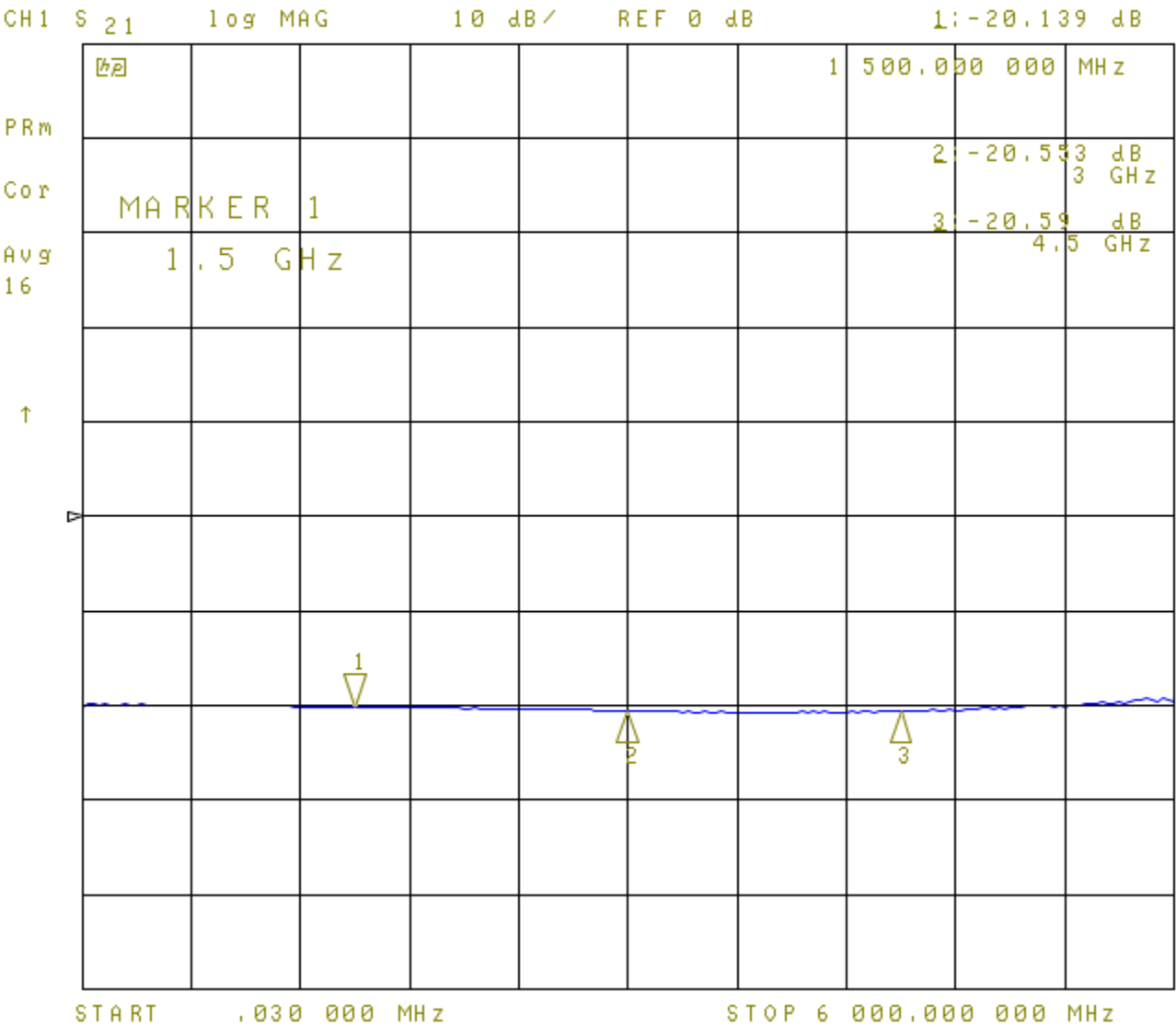
20dB Attenuator, S21
