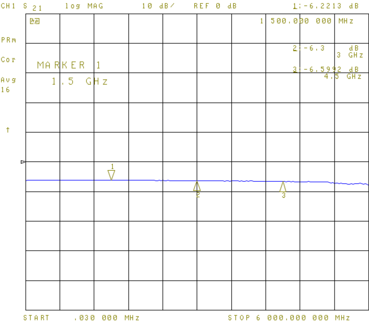
6dB Attenuator, S21
