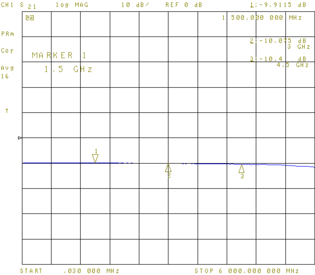
10dB Attenuator, S21
