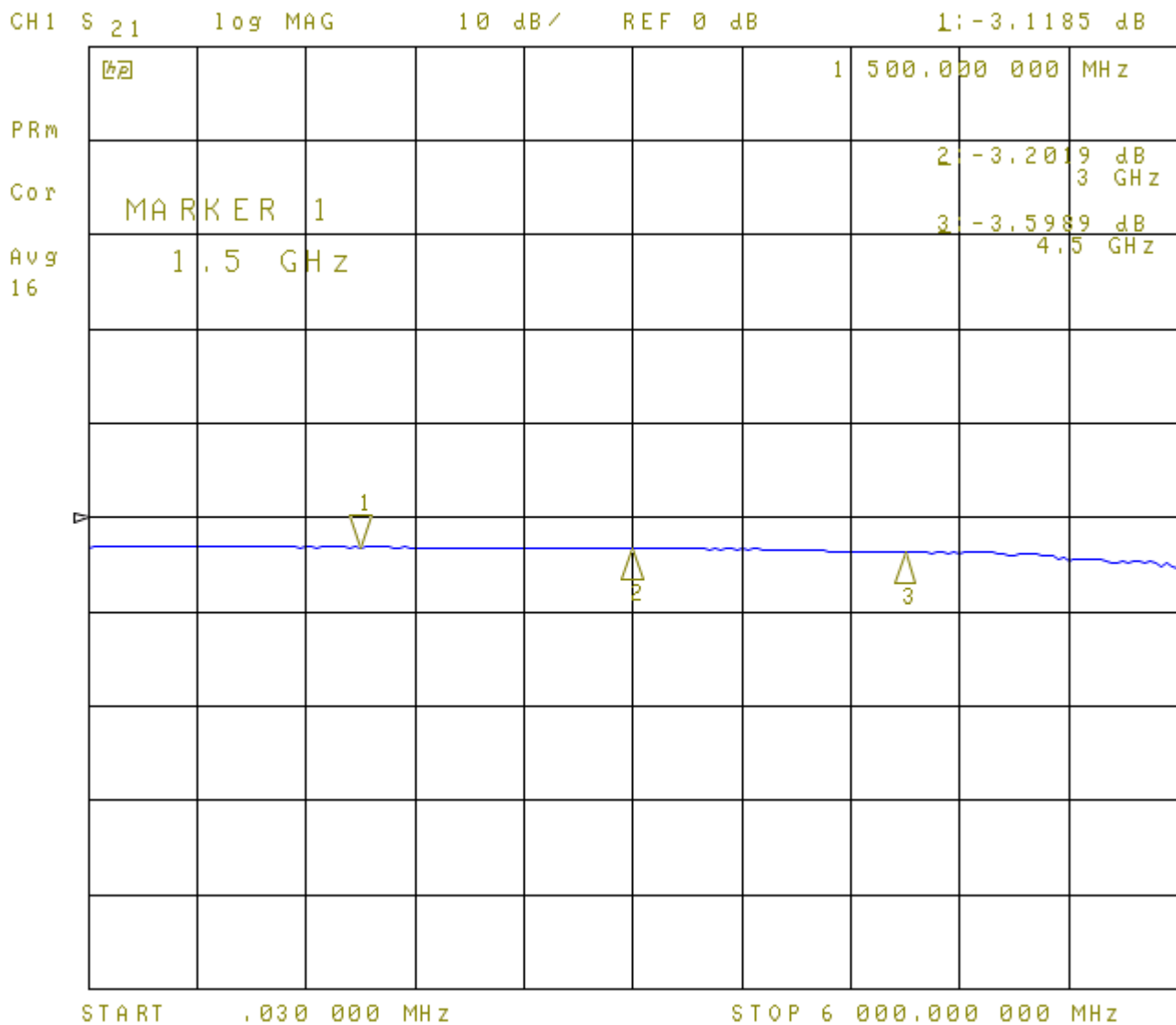
3dB Attenuator, S21
