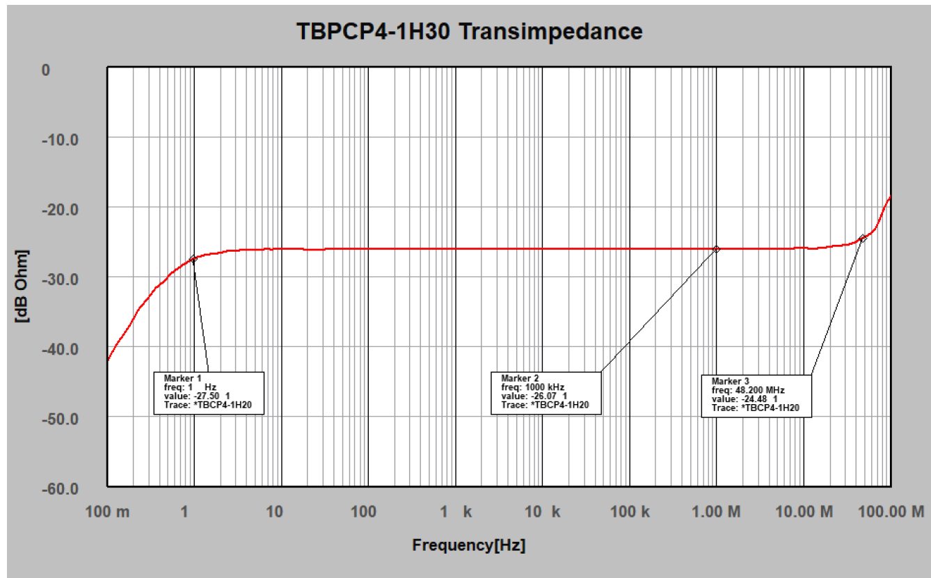
Figure1: typical transfer impedance, 1 Hz – 100 MHz
