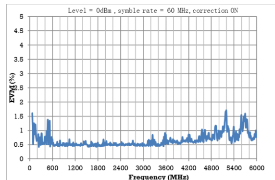
Measured EVM performance vs carrier frequency@ symbol rate=60 MHz, QPSK
