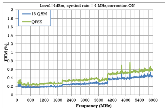
Measured EVM performance vs carrier frequency@ symbol rate=5 MHz
