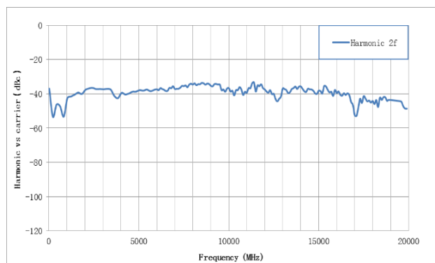
Second harmonic versus carrier frequency at level \leq + 10 \text{ dBm}
