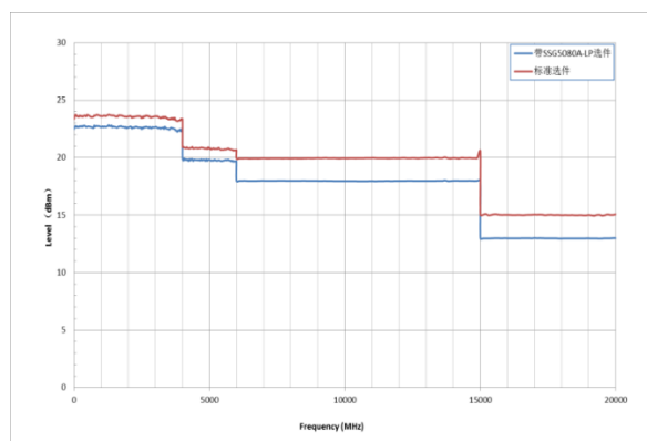
Maximum output power versus frequency, f \geq 1\text{ MHz}
