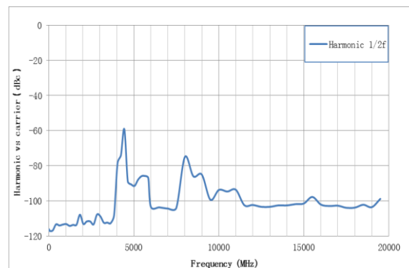
Sub harmonic versus carrier frequency at level \leq + 10 \text{ dBm}
