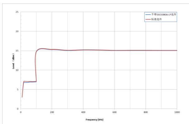
Maximum output power versus frequency, f < 1\text{ MHz}
