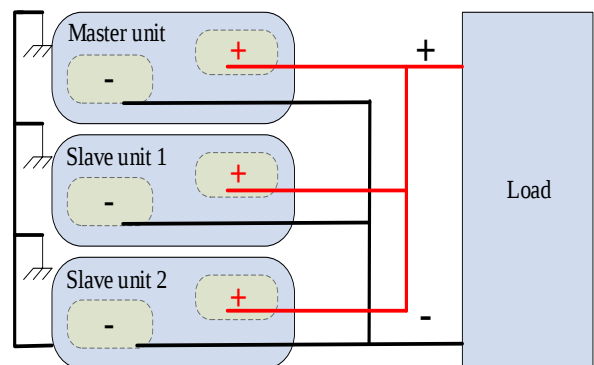
Parallel Connection
