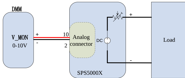
External DMM Monitoring of the Output Voltage
