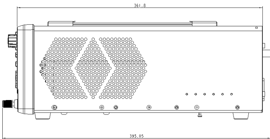
Right View (SPD4121X/SPD4306X)
