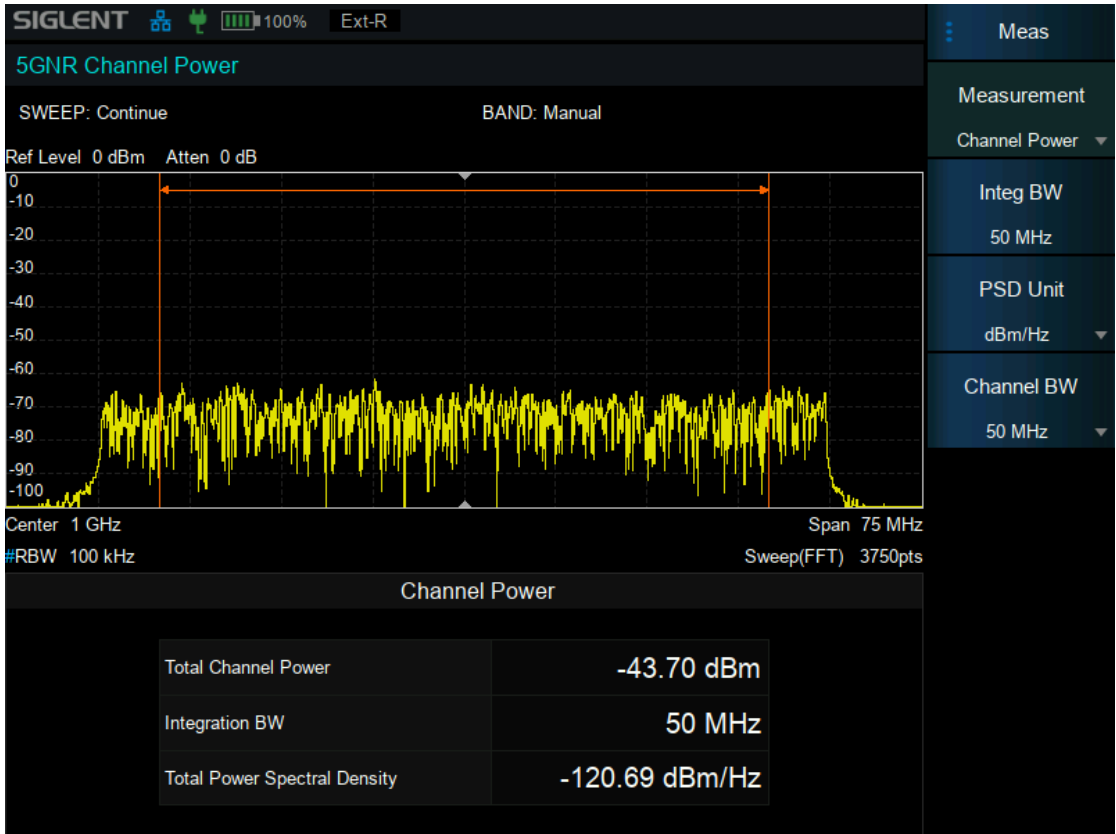
Figure 8–5 Channel power view
