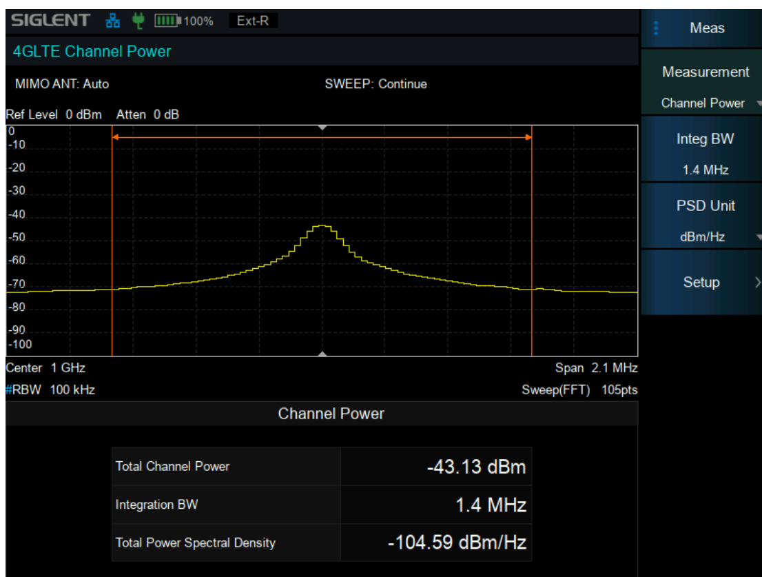
Figure 9–4 Channel Power View
