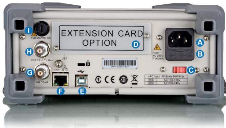
Figure 2 Rear Panel
