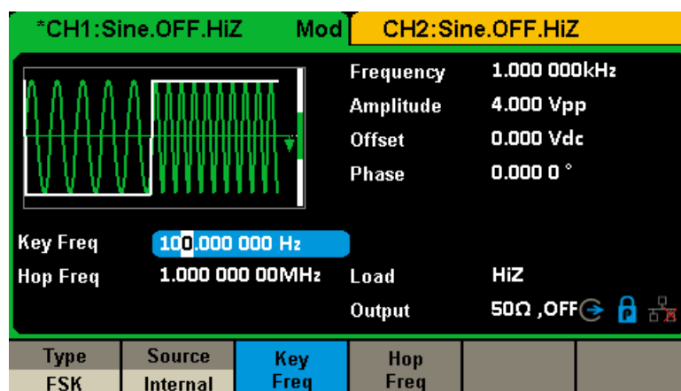
Figure 2-28 Setting Interface of FSK Modulation
