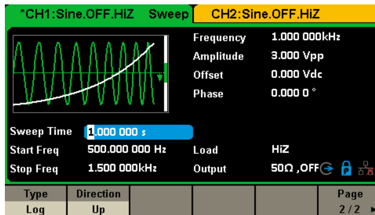
Figure 2-37 Log Sweep Interface
