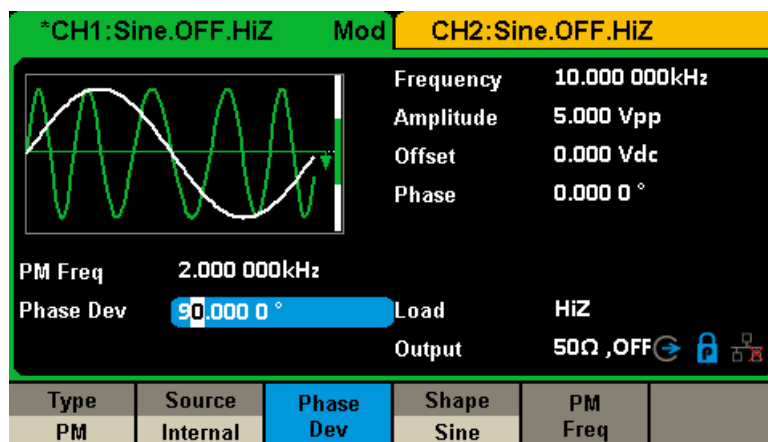
Figure 3-11 Generate a PM Modulation Waveform
