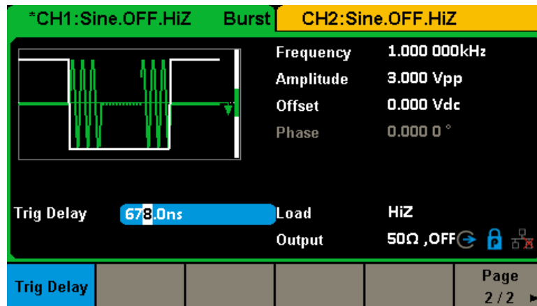
Figure 2-42 Gated Burst Interface (Page 2/2)
