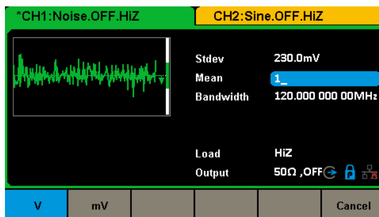
Figure 2-15 Setting the Mean
