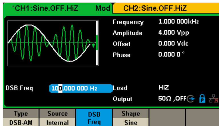
Figure 2-25 Setting Interface of DSB-AM Modulation
