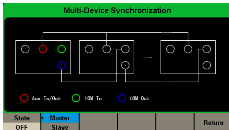
Figure 2-86 Multi-Device Sync Interface
