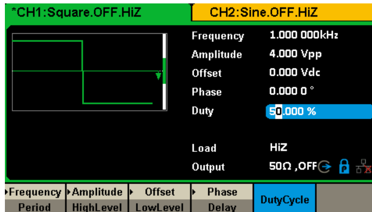
Figure 2-6 Square Parameters Display Interface
