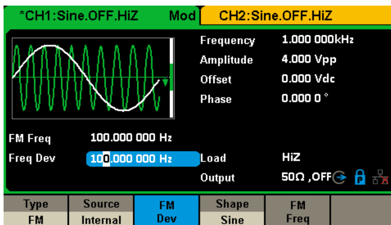
Figure 2-26 Setting Interface of FM Modulation
