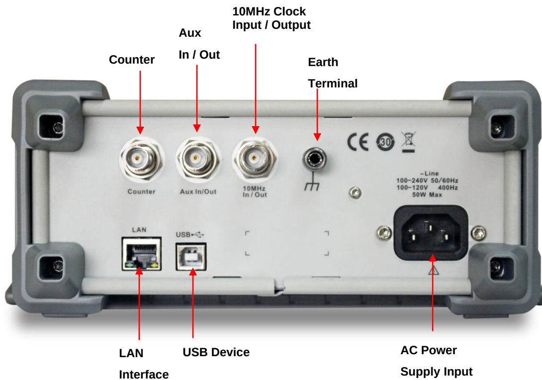
Figure 1-3 Rear Panel of SDG2000X
