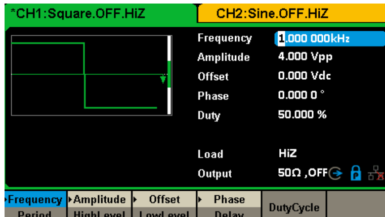
Figure 1-7 Square Display Interface
