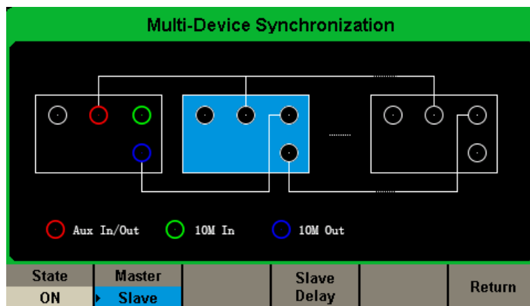
Figure 2-88 Slave mode Interface
