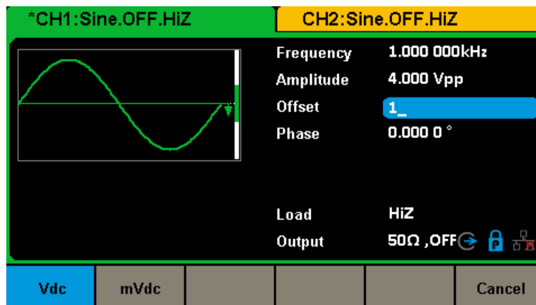
Figure 2-4 Setting the Offset
