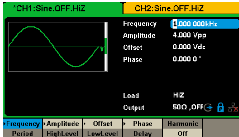
Figure 2-83 Phase-locked Mode
