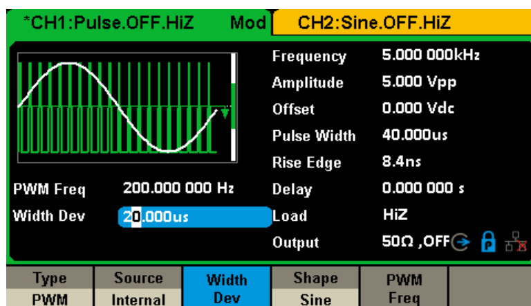
Figure 3-15 Generate a PWM Modulation Waveform
