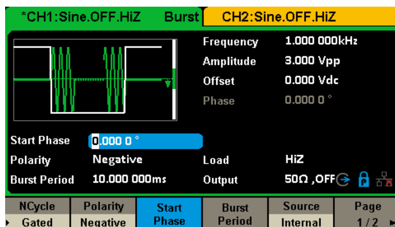
Figure 2-41 Gated Burst Interface (Page 1/2)
