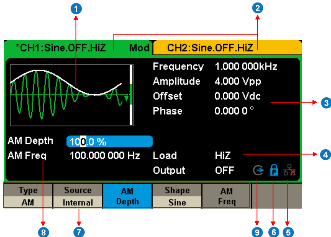
Figure 1-4 Touch Screen Display
