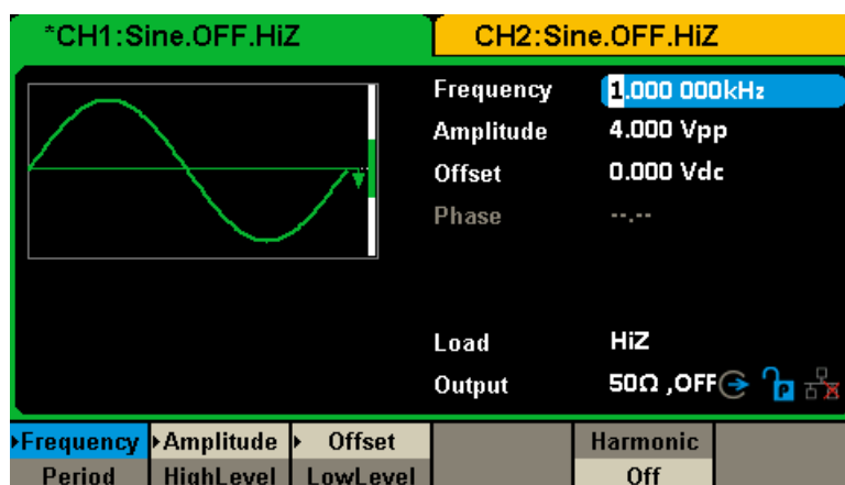
Figure 2-84 Independent Mode
