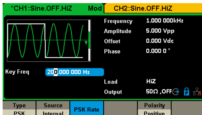
Figure 3-14 Generate a PSK Modulation Waveform
