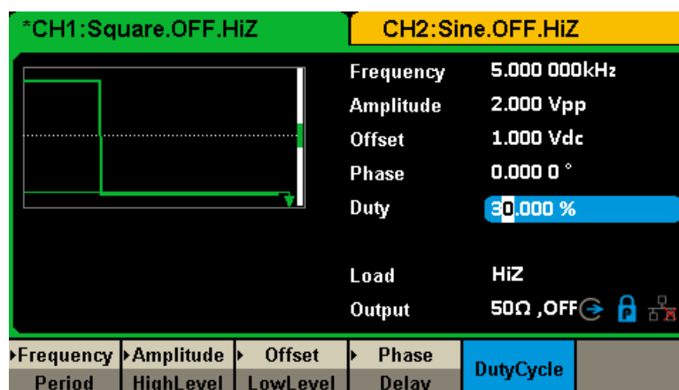
Figure 3-2 Generate a Square Waveform
