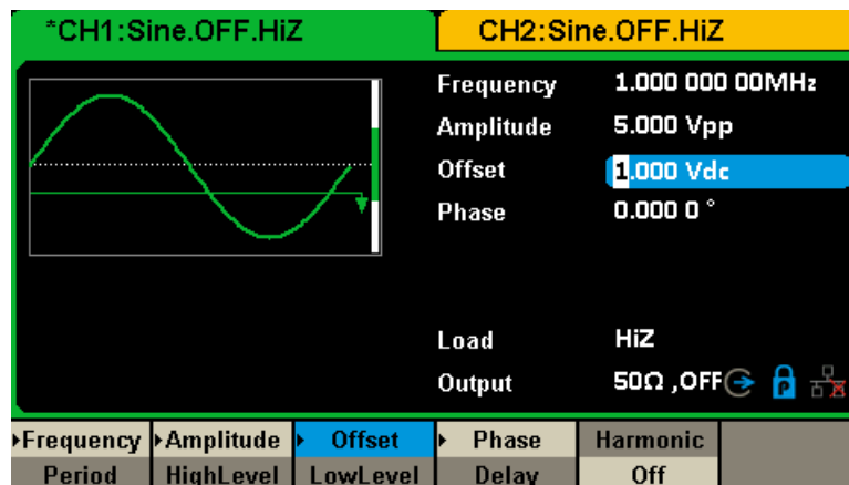
Figure 3-1 Generate a Sine Waveform
