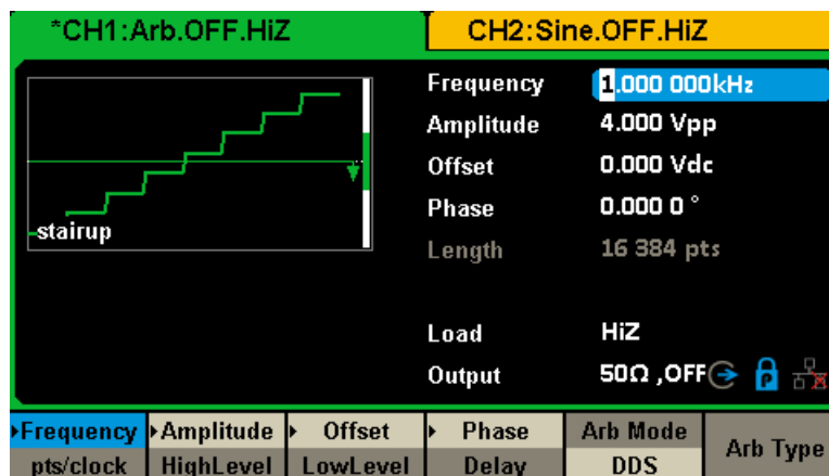
Figure 1-12 Arbitrary Waveform Display Interface
