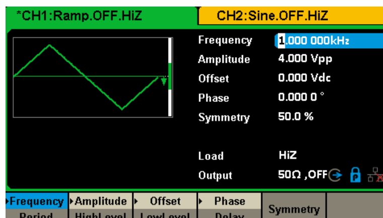
Figure 1-8 Ramp Display Interface
