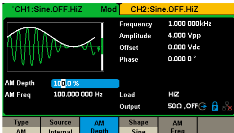
Figure 1-14 Modulation Display Interface
