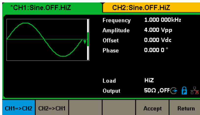
Figure 2-72 Channel Copy Interface
