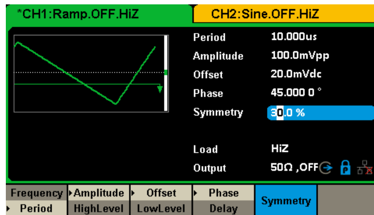
Figure 3-3 Generate a Ramp Waveform
