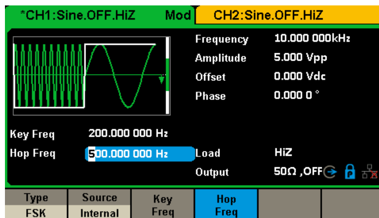
Figure 3-12 Generate a FSK Modulation Waveform
