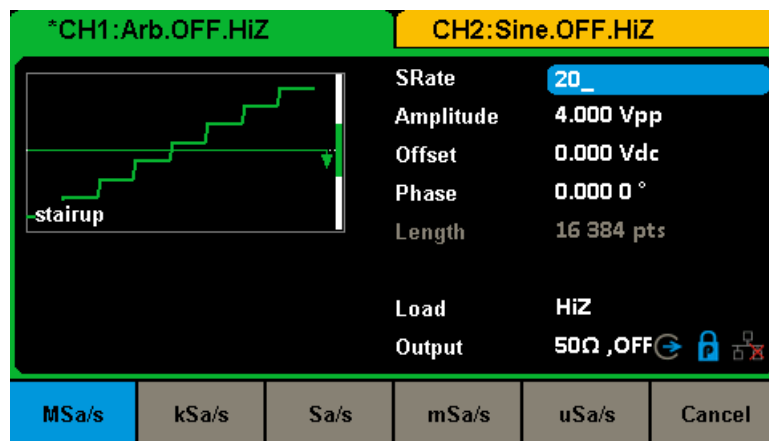
Figure 2-20 Setting the Sampling Rate
