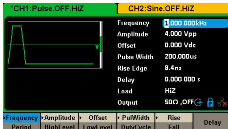
Figure 1-9 Pulse Display Interface
