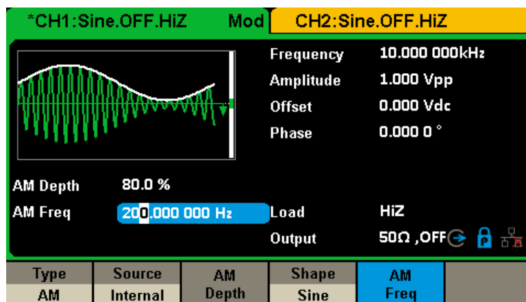
Figure 3-9 Generate an AM Modulation Waveform
