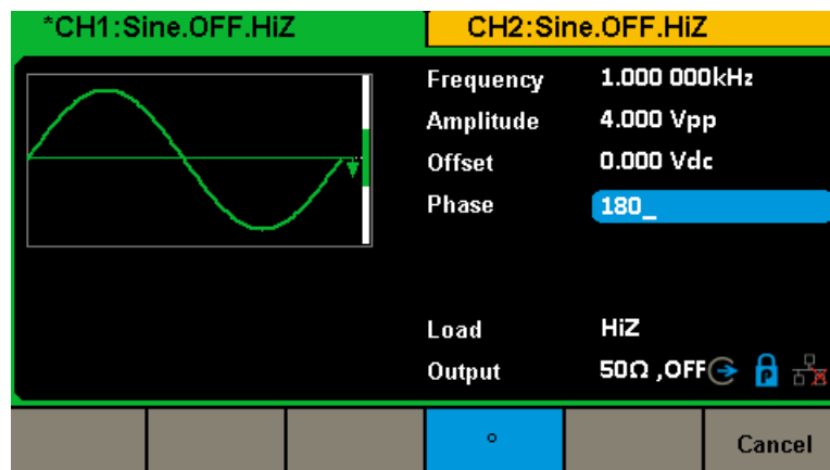
Figure 2-5 Setting the Phase
