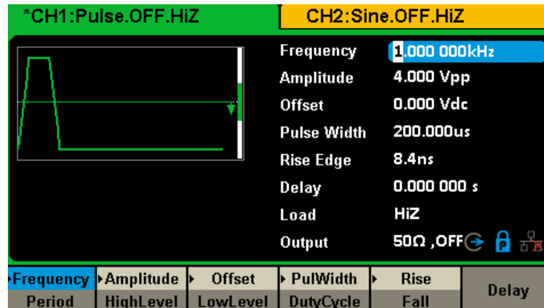
Figure 2-10 Pulse Parameters Display Interface
