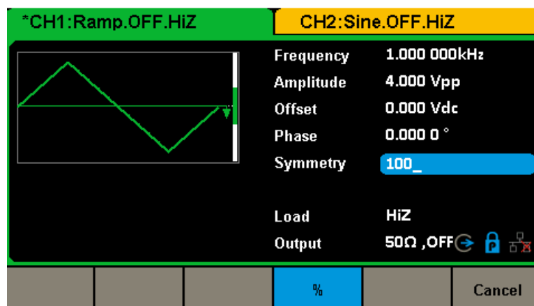
Figure 2-9 Setting the Symmetry
