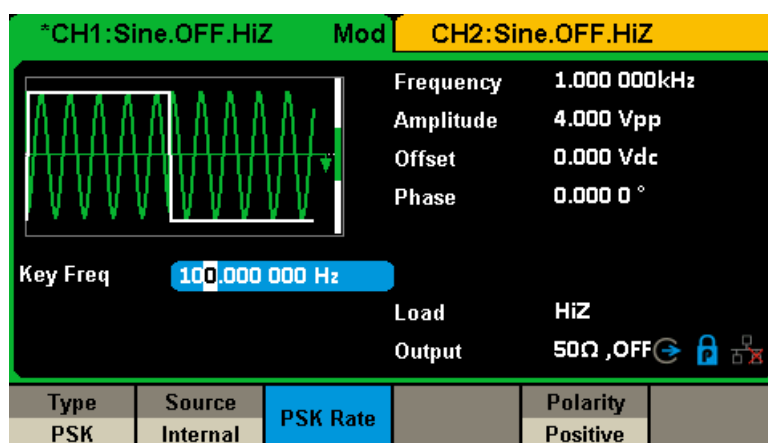
Figure 2-30 Setting Interface of PSK Modulation
