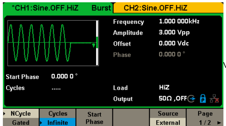
Figure 2-40 Infinite Burst Interface
