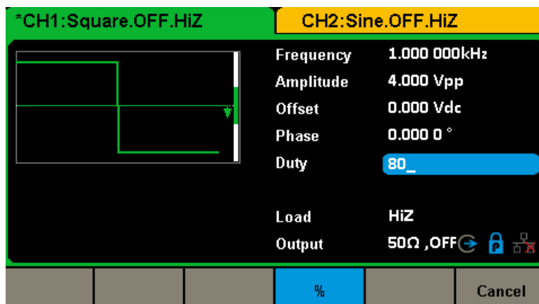
Figure 2-7 Setting the Duty Cycle
