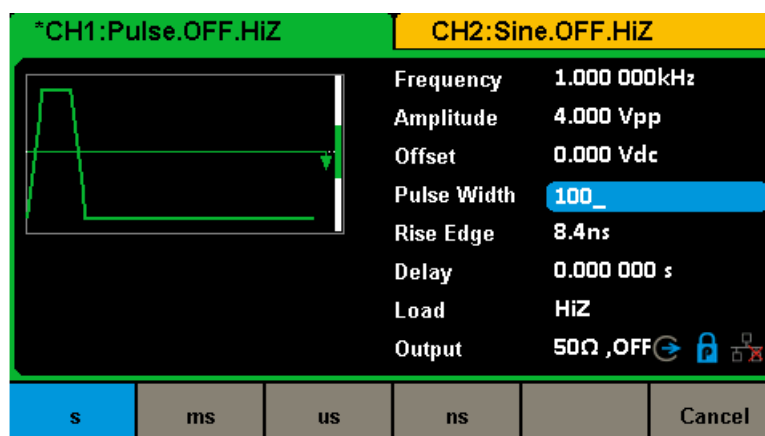
Figure 2-11 Setting the Pulse Width
