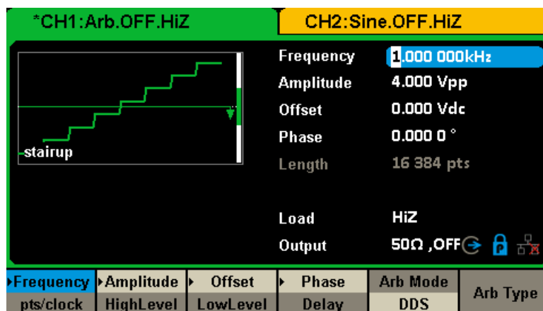
Figure 2-18 Arb Parameters Display Interface (DDS)
