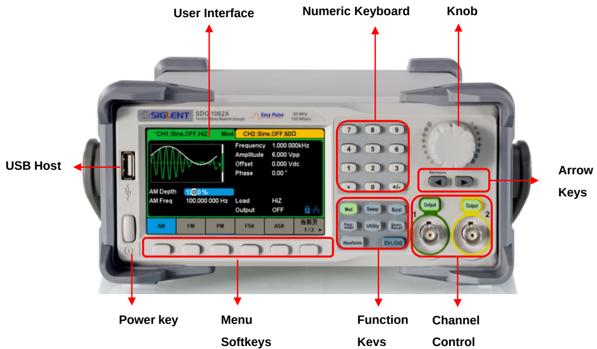
Figure 1-2 Front Panel of SDG2000X
