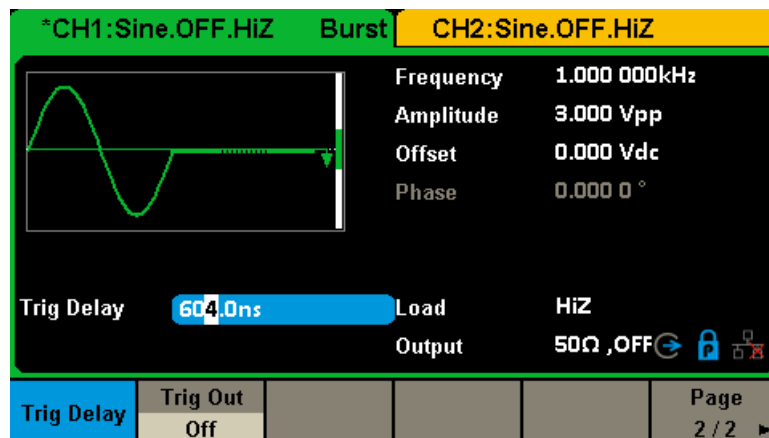
Figure 2-39 N-Cycle Burst Interface (Page 2/2)
