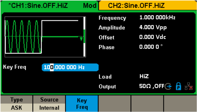
Figure 2-29 Setting Interface of ASK Modulation
