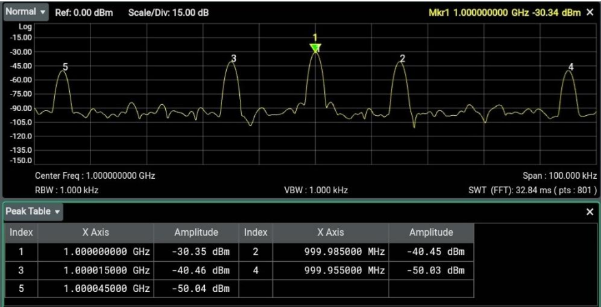
Figure 5.13 Peak Table
