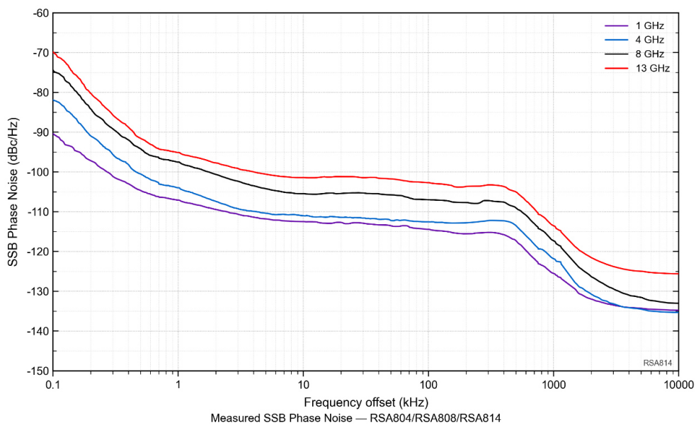
Measured SSB Phase Noise — RSA804/RSA808/RSA814
