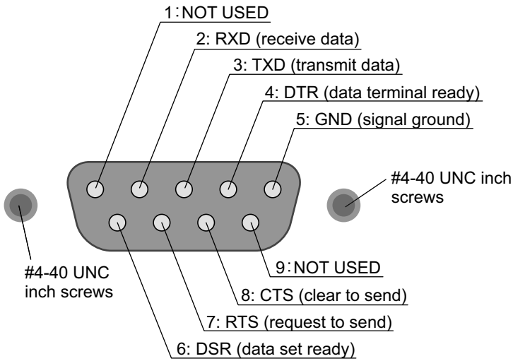
RS232C pinout (viewed from the product's rear panel)
