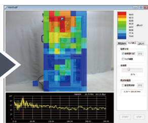
- Big-size probes - Large equipment EM field measurement
