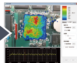
- Small precision probes - Small components and PCB EM field measurement
