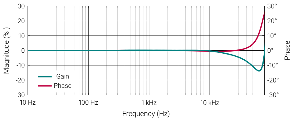
Figure 3: Frequency characteristics
