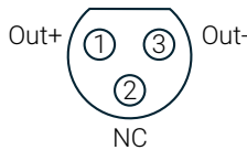
Figure 7: XLR Mini voltage reading output pinout
