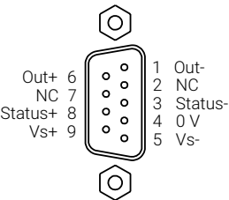
Figure 7: D-sub-9 connection pinout
