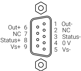
Figure 7: D-sub-9 connection pinout
