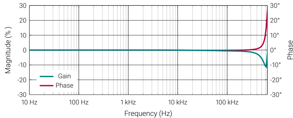
Figure 4: Frequency characteristics
