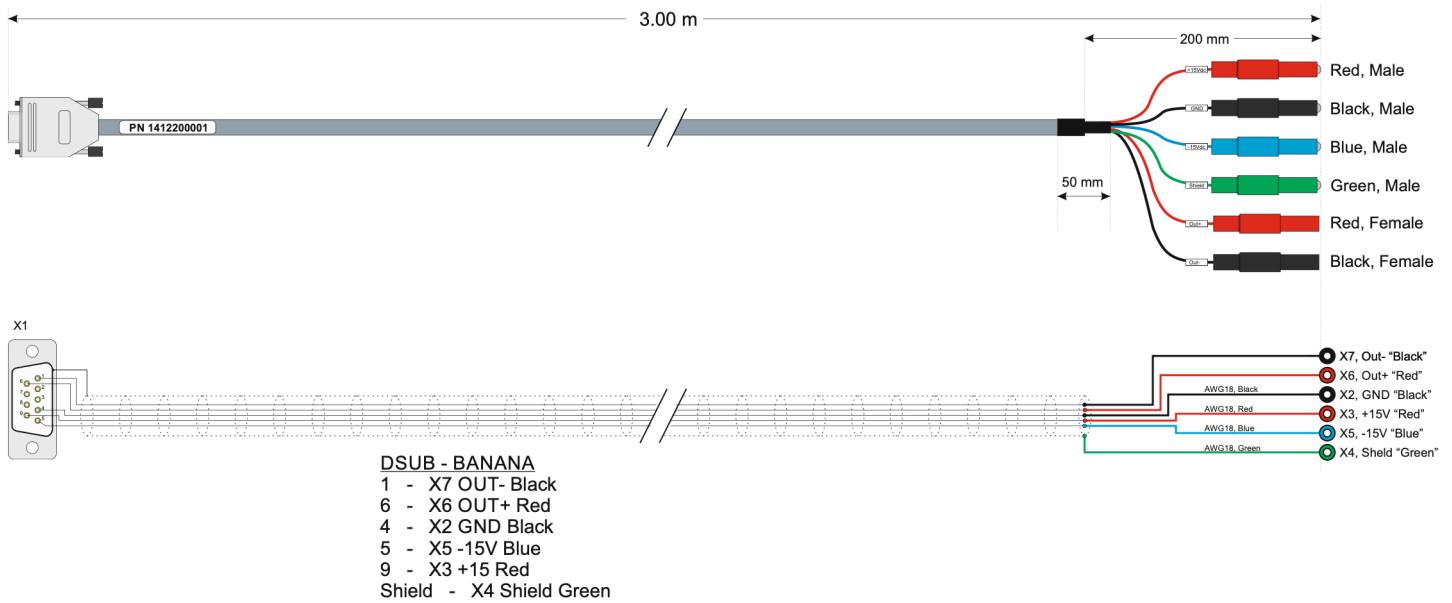
Part number: 1412200001- DS-ID Power and signal cable 3m
