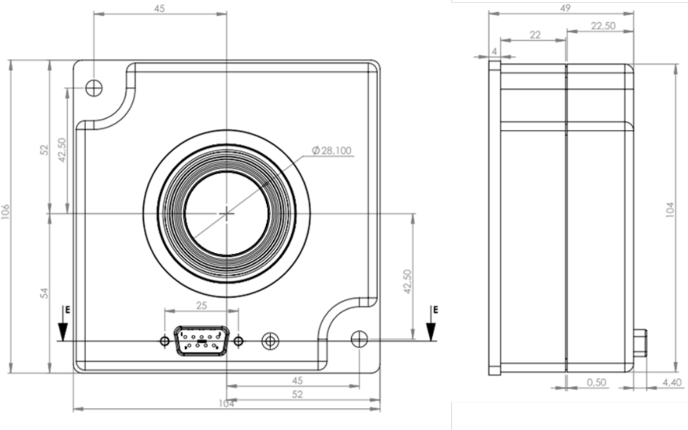
Figure 5: Dimensions of sensor head. Tolerance is 0.3 mm
