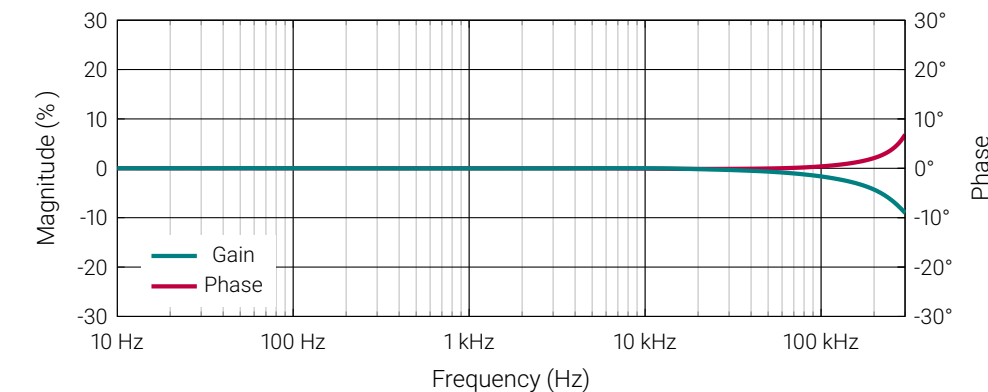
Figure 4: Frequency characteristics
