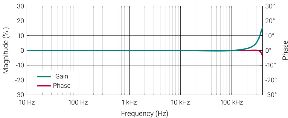
Figure 4: Frequency characteristics
