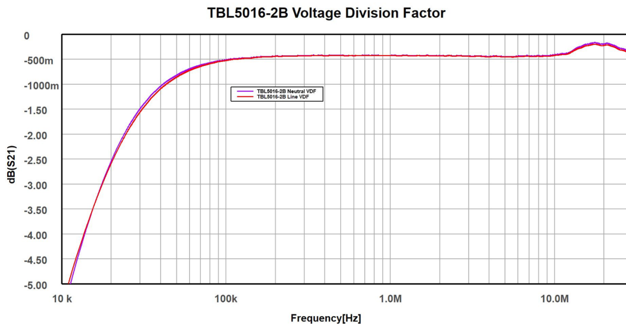
Voltage Division Ratio versus frequency, typ.
