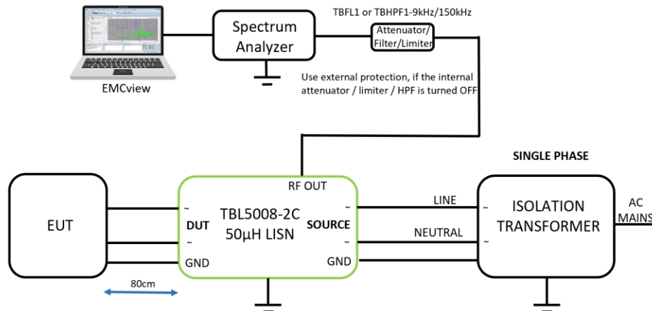
Basic wiring diagram for conducted emission measurements
