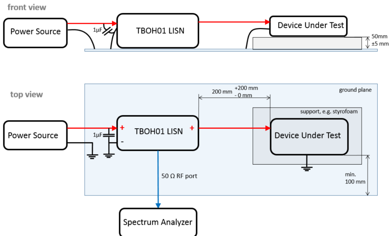
CISPR 25, voltage method, EUT (DUT) locally grounded
