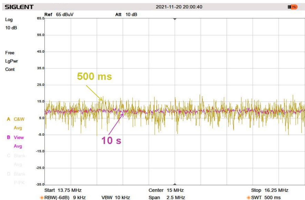
Analyzer base noise (DANL) with 500 ms sweep time versus 10 s sweep time
