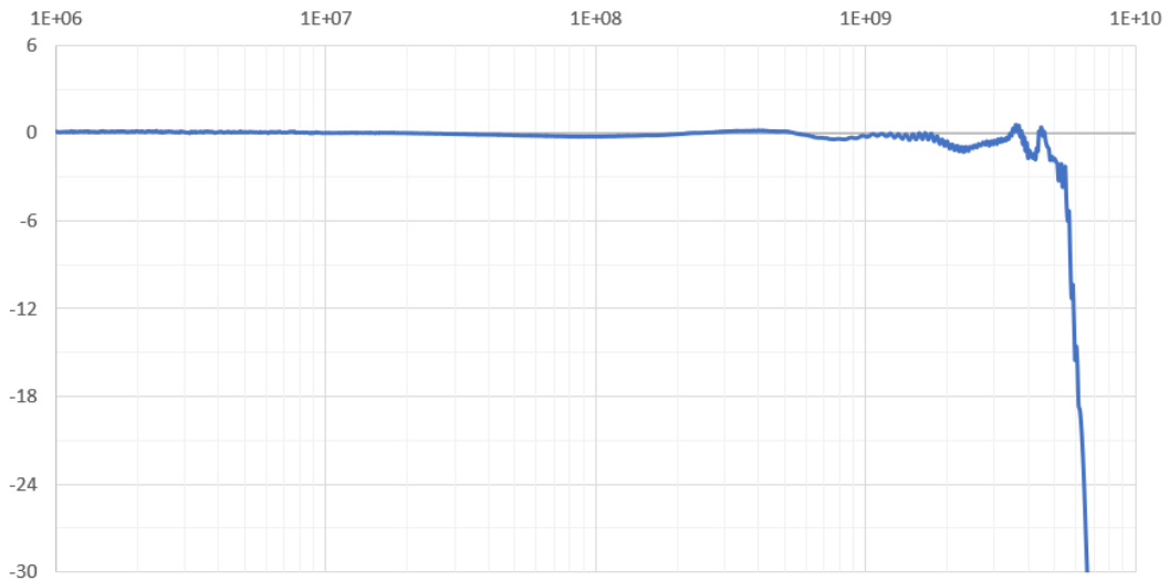
SSI-50 frequency response curve (welding 24.9R resistor)
