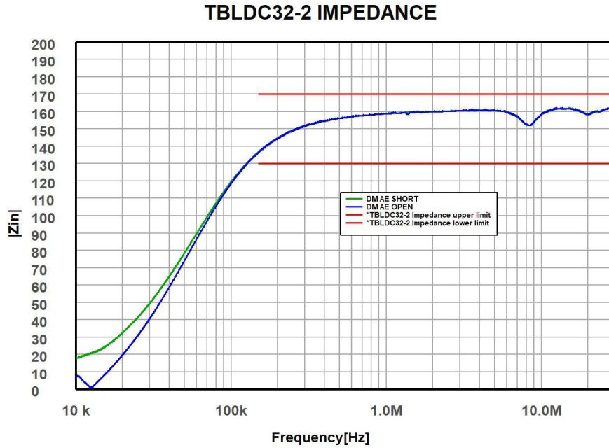
Figure 7 – Impedance [Ω] vs. frequency at EUT terminals, DM, AE terminals open / shorted
