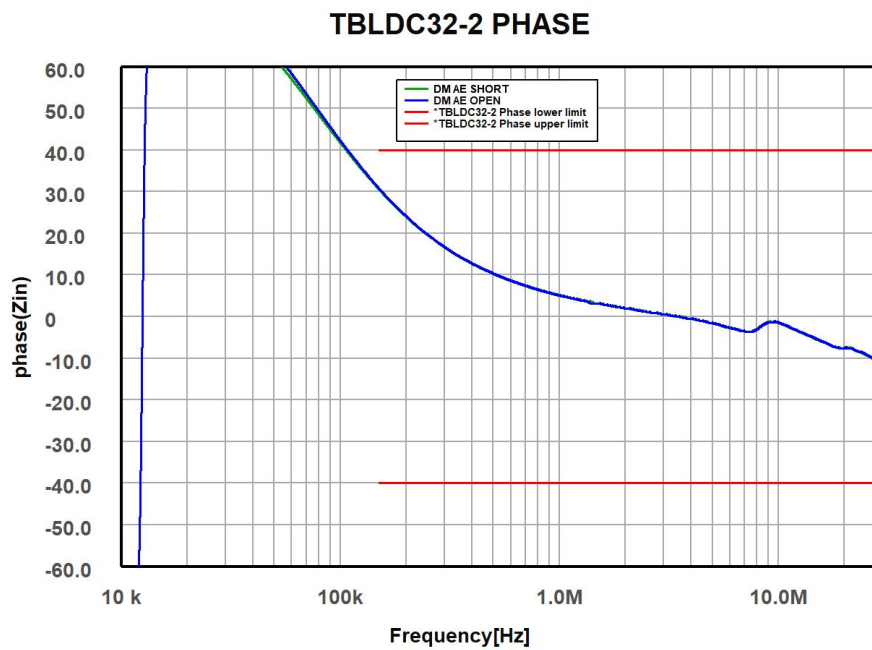
Figure 8 – Phase angle [°] vs. frequency at EUT terminals, DM, AE terminals open / shorted
