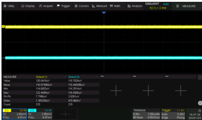
Low noise floor: 125 µVrms at 1 GHz bandwidth
